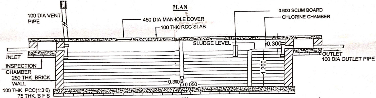
SECTION SEPTIC TANK DETAILS (FOR 100 USERS / VOLUME : 17 CUM.) (SCALE - 1:50)
